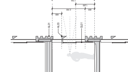
7 SECTION FT2.1 - Flush SI
