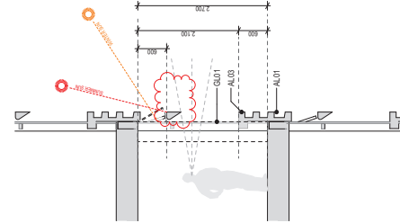
7 SECTION FT2.1 - Flush SI
