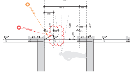
9 SECTION FT2.3 - Wind Affected SI
