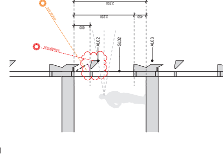
3 SECTION FT1.3 - Wind Affected SI
