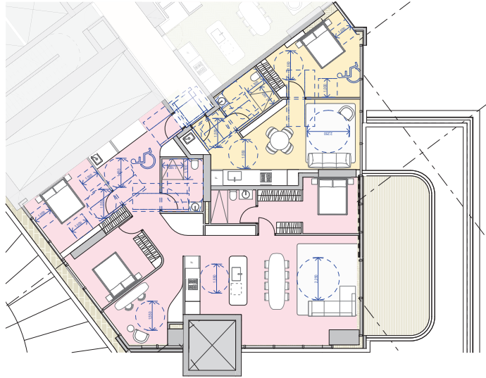
2 PLAN Level 12 Post-Adaptable 1:100
