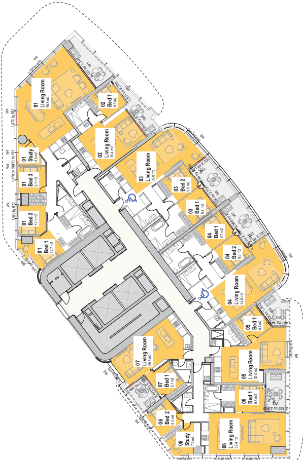
PLAN Level 18 to 21 1:150
