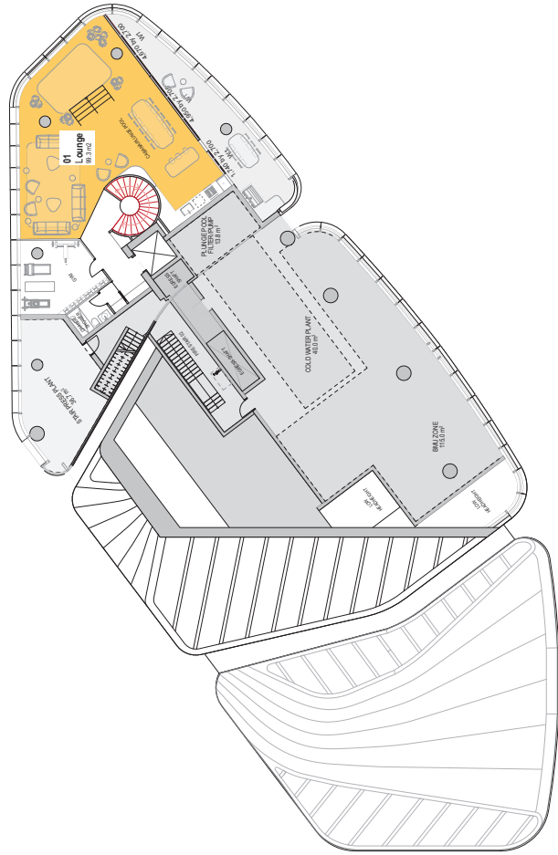
03 PLAN Level 53 - Penthouse / Plant 1:150
